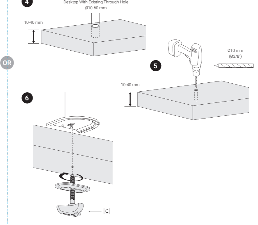
03 Grommet Mounting
