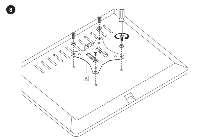
01 Clamp Mounting
