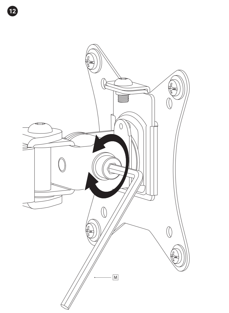
08 Screen Regulation
